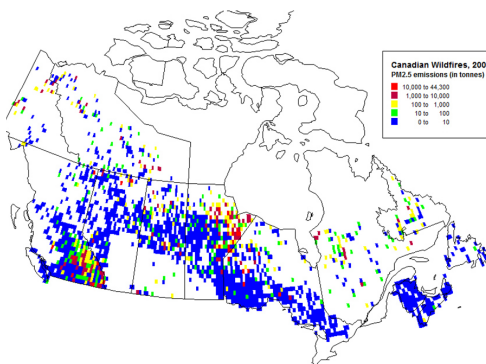
Figure 1. Gridded PM 2.5 emission amounts from wildfires.
