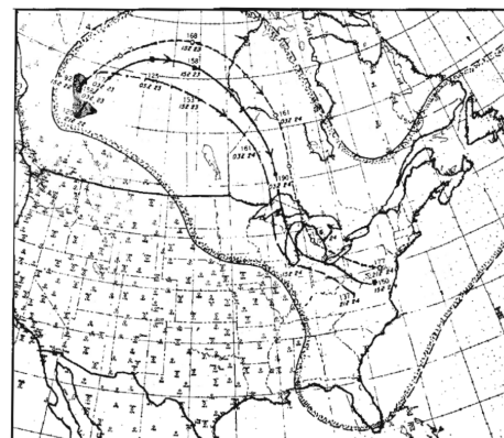
Figure 3. Extent of smoke, based on a special survey of weather stations 10 commissioned by Harry Wexler.
