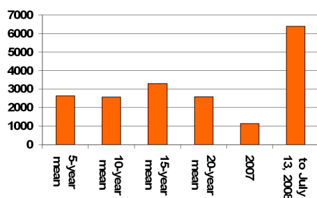
Figure 1. Area burned (km 2 ) in Saskatchewan
